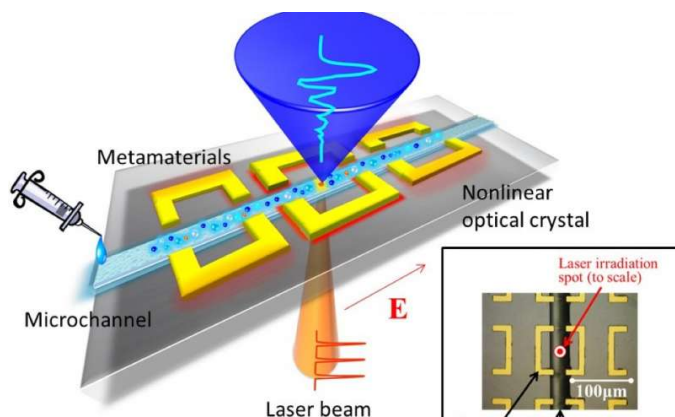
Fig.1. A schematic drawing of solution measurement by using fabricated terahertz microfluidic chip. The chip consists of a local THz radiation point source, a single microchannel and a few arrays of split ring resonators. The THz waves are ... more
