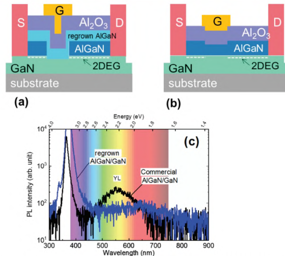
FIG. 1. Schematic illustration of (a) proposed recessed-gate with regrown barrier GaN-based MIS-HEMT and (b) conventional recessed-gate GaN-based MIS-HEMT. (c) PL spectra of regrown AlGa N /GaN and commercial AlGa N /GaN.
