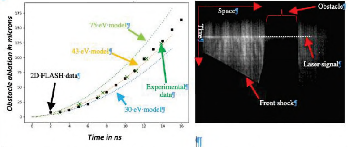
Fig. 1. On the left, an example of a comparison between the obstacle ablation due to radiation of the shock for a 150 mbar of xenon (green crosses), data from a 2D FLASH simulation (black squares) and our theoretical model (dotted colored curves) for different shock temperatures. Right picture is a typical example of result given by the streak camera of the shadowgraphy diagnostic.
