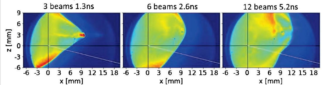
FIG. The upper panels show experimental setup. The lower panels denote GOI images of self-emission at t = 110 ns for different laser energy (same intensity): (left) 1.4 kJ, (middle) 2.8 kJ, (right) 5.6 kJ, respectively.
