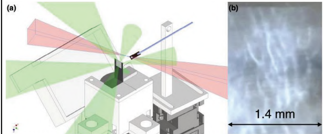
FIG. (a) Mechanical drawing of the experimental setup. Three GXII beams (green) irradiate the Al planar target to produce a fast directional plasma flow, and one GXII beam from the top also irradiates the Al slab target on the bottom to create two-plasma interaction. LFEX laser (red) irradiates an LSG target with defocused intensity. The accelerated ions are detected with SSNTD. (b) Ion radiograph at 10 ns from GXII laser irradiation (partial image) shows wave-like structures.
